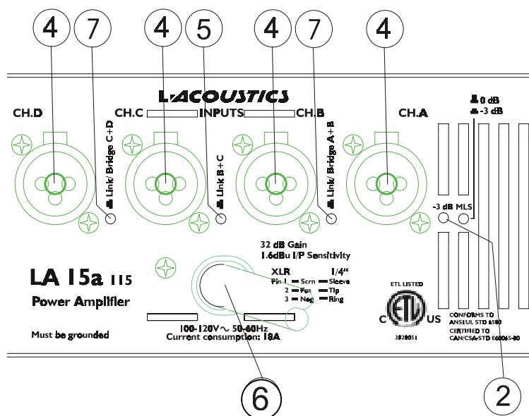
図 3: LA15a Rear Panel MLS Switches
