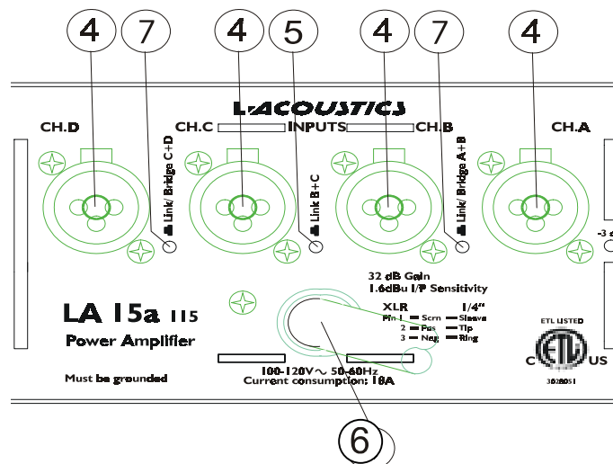
図 7: LA15a Rear Panel Detail
