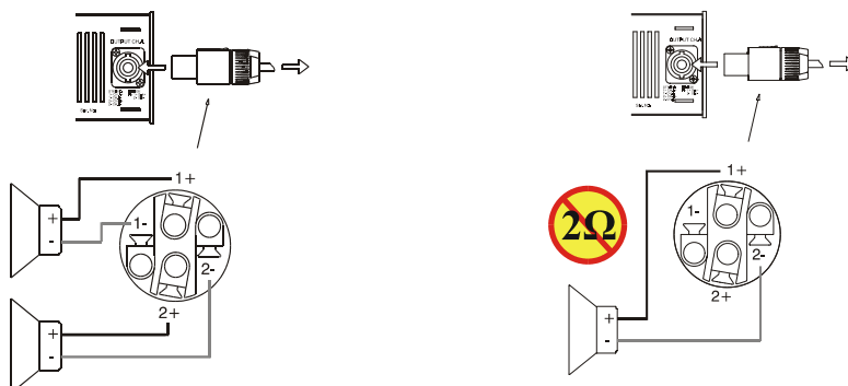
図 10: Loudspeaker Connection Details
