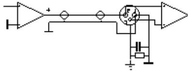
図 8: Unbalanced Line Connection
