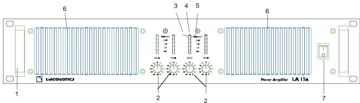
図 1: LA15a Front Panel
