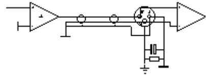
図 9: Balanced Line with Unbalanced Equipment
