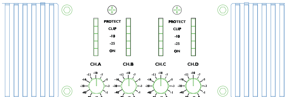
図 13: LA15a Front Panel Detail
