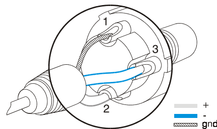
図 5: Balanced XLR wiring
