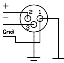
図 4: XLR Input Connector Wiring
