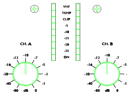
図 13: LA48a Front Panel Detail
