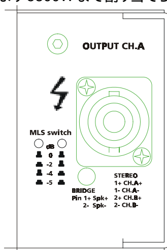
図 3: LA48a Rear Panel MLS Switches
