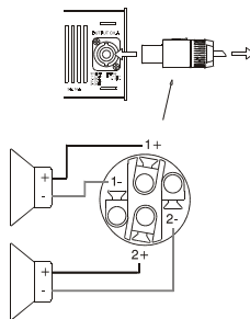
図 10: Loudspeaker Connection Details
