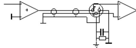
図 9: Balanced Line with Unbalanced Equipment
