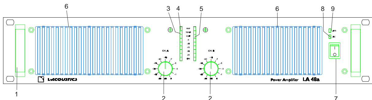
図 1: LA48a Front Panel
