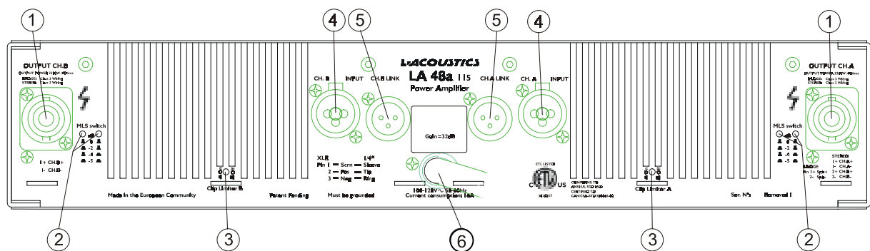
図 2: LA48a Rear Panel
