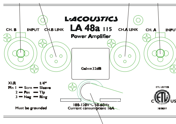
図 7: LA48a Rear Panel Detail
